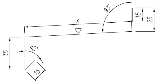
O05 Horizontal bottom window flashing
